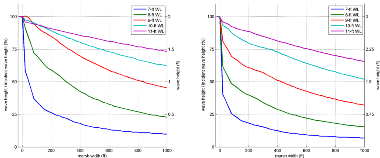
Figure 18. Predicted wave heights relative to incident wave height as a function of marsh width, from the WHAFIS model (see section 7).The incident wave height equals (a) 2 feet and (b) 3ft (BCDC 2013).
